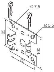
525.10029 Support universel
