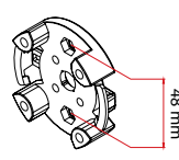
Support renforcé
